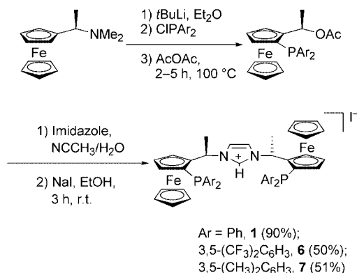
Scheme 2. Synthesis of the ligand precursors 1 , 6 , and 7 .
