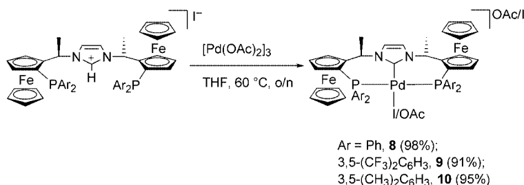
Scheme 3. Synthesis of the palladium complexes 8 , 9 , and 10 .
