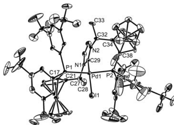
Figure 2. ORTEP representation of the cation in [\text{PdI}(3,5\text{-CF}_3\text{-PCP})]\text{PF}_6 ( 14 ). Hydrogen atoms are omitted for clarity. Thermal ellipsoids are set to 30% probability.
