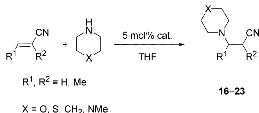
Scheme 5. Hydroamination of cyano olefins.
