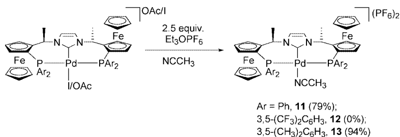
Scheme 4. Synthesis of the dicationic complexes 11 and 13 .
