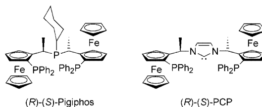
Scheme 1. The C 1 -symmetric triphosphane Pigiphos and a structurally related C 2 -symmetric PCP ligand.
