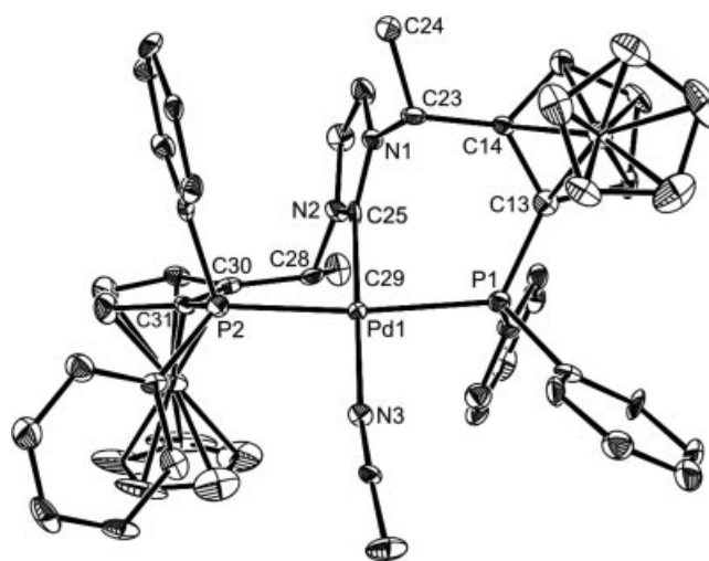
Figure 3. ORTEP representation of the dication in [Pd(NCCH 3 )(PCP)](PF 6 ) 2 ( 11 ). Hydrogen atoms are omitted for clarity. Thermal ellipsoids are set to 30% probability.
