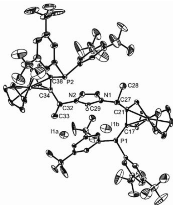
Figure 1. ORTEP representation of (3,5- \text{CF}_3 -PCPH)I ( 6 ). Hydrogen atoms and the \text{CF}_3 disorder are omitted for clarity. Thermal ellipsoids are set to 30% probability.
